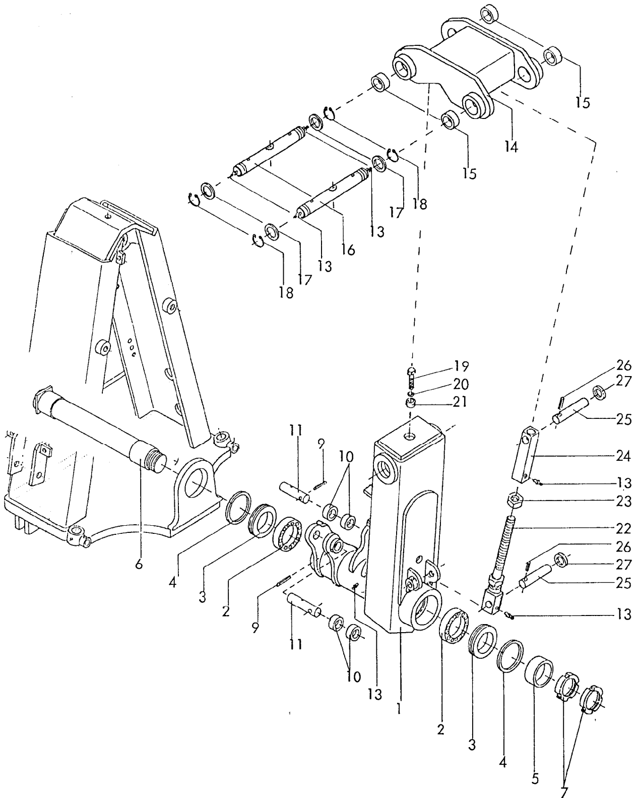
4766 / 4767 Kranich, Kranich-Avant 180 A, AS Baureihe 3 -Wendearm- 04.89
