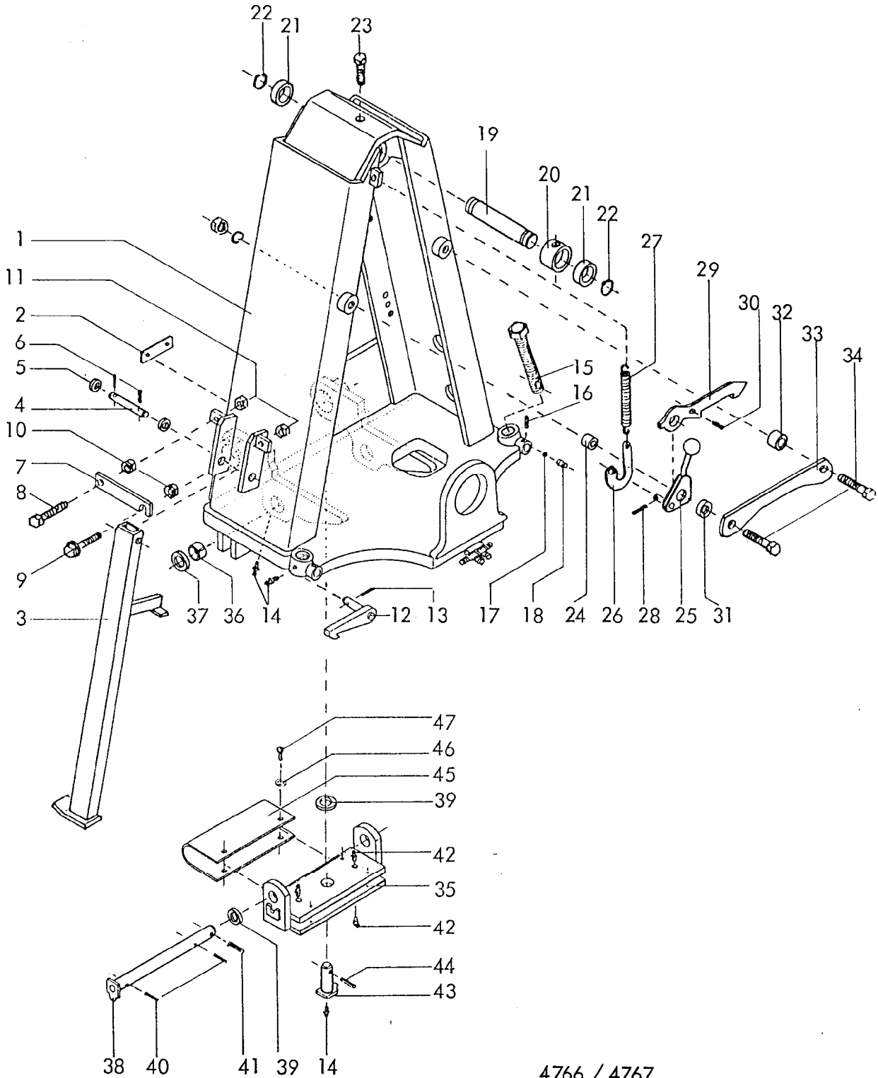
4766 / 4767 Kranich, Kranich-Avant 180 A, AS Baureihe 1, 2, 3 -Traverse- 04.89
