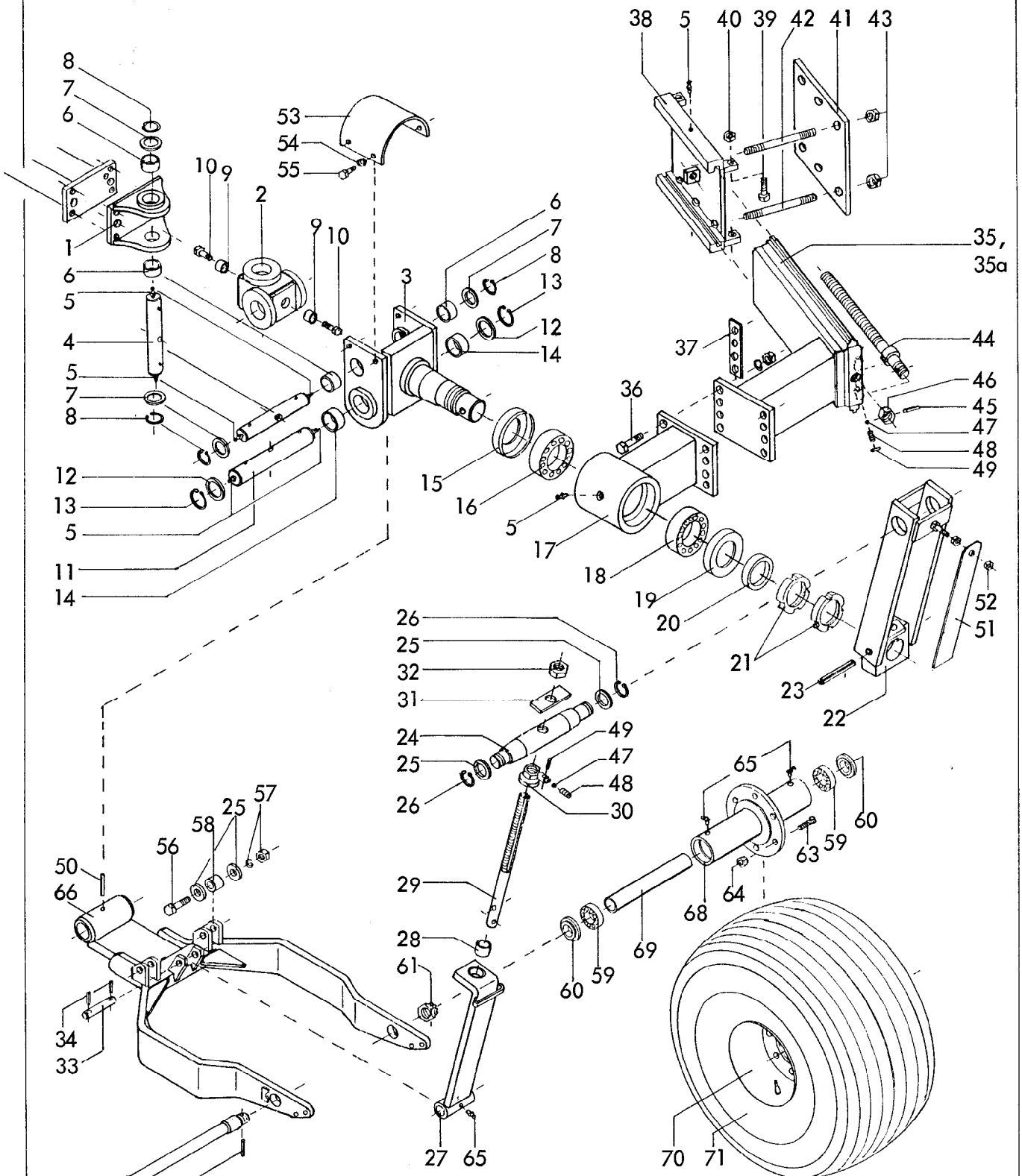
4766 / 4767 Kranich, Kranich-Avant 180 A, AS Baureihe 3 -Hinterrad- 04.89
