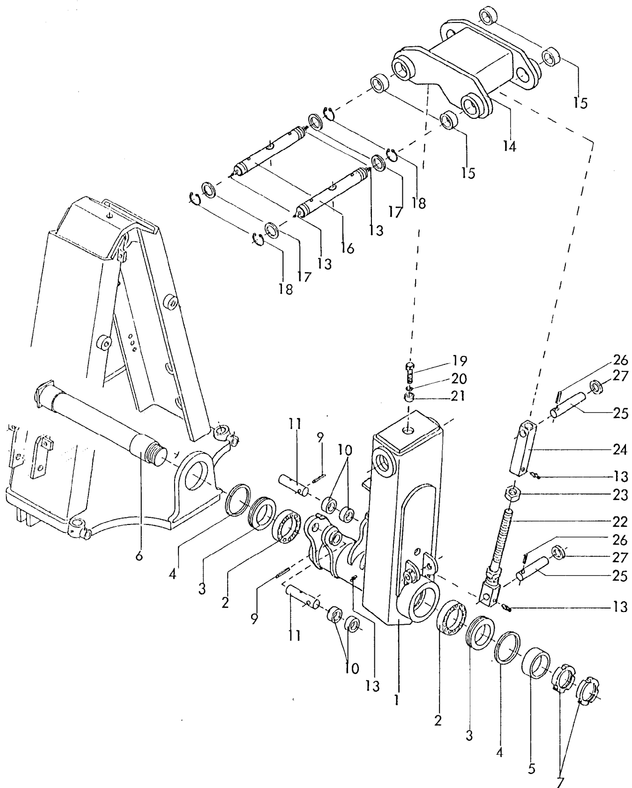
4766 / 4767 Kranich, Kranich-Avant 180 A, AS Baureihe 1, 2 -Wendearm- 10.88
