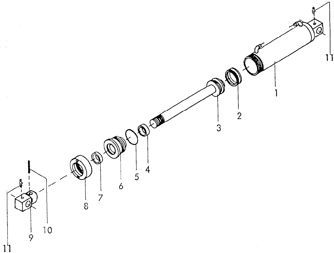
Kranich, Kranich-Avant 180 A, AS Baureihe 1, 2
