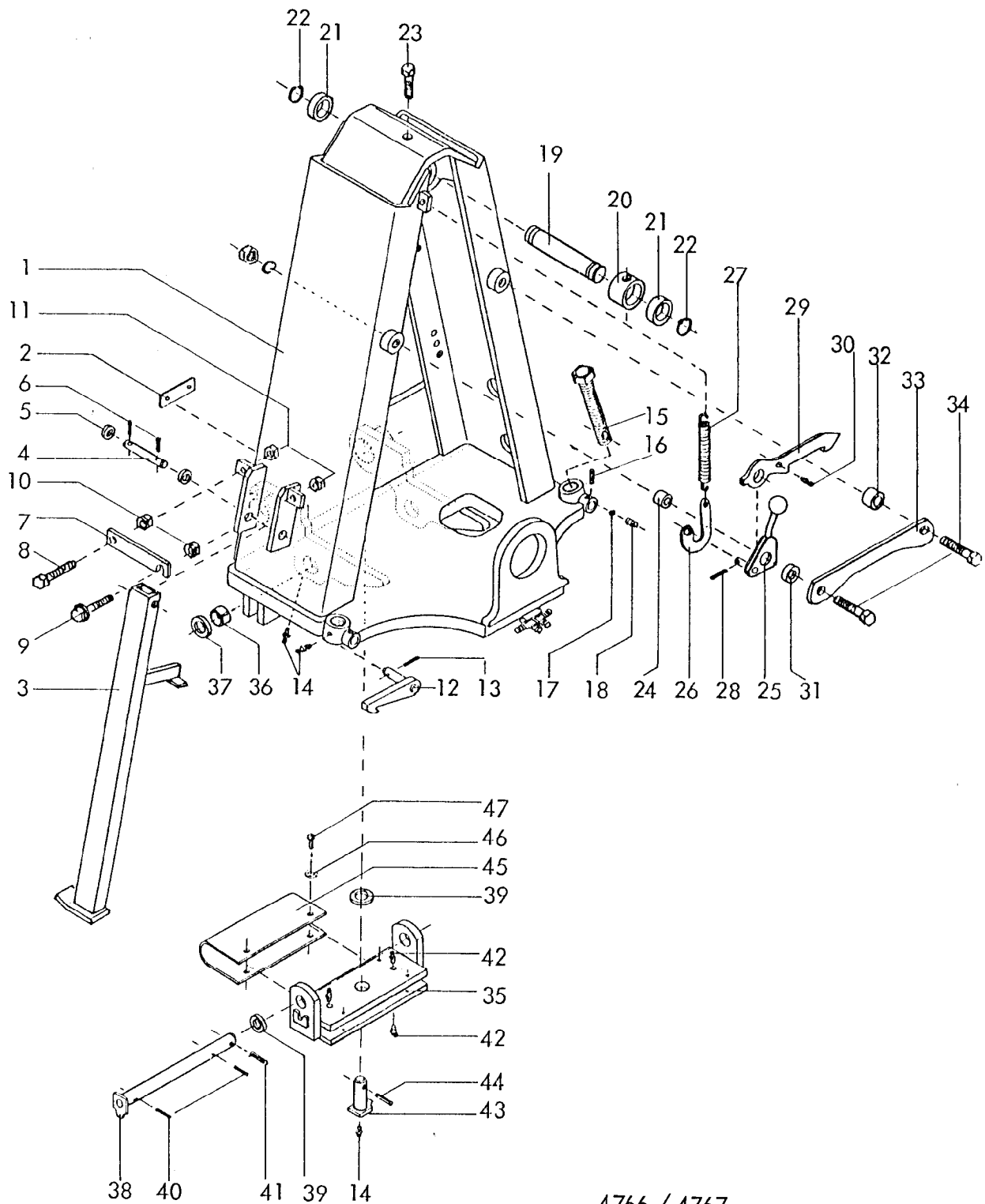
4766 / 4767 Kranich, Kranich-Avant 180 A, AS Baureihe 1, 2 -Traverse- 10.88
