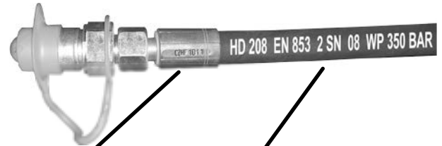
Fig. 90; Identification Flexible hydrauliques
